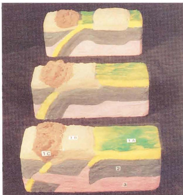
Figure 12: A model illustrating how a lithosphere plate (rawāsi) (2) with the oceans (1A) and the continents (1B) sink into the earth under the leading edge of another plate (see upper and middle models). The lower model shows how the mountain range (1C), acting as a wedge between the plates, prevents the continent-bearing lithosphere from sinking into the earth.
